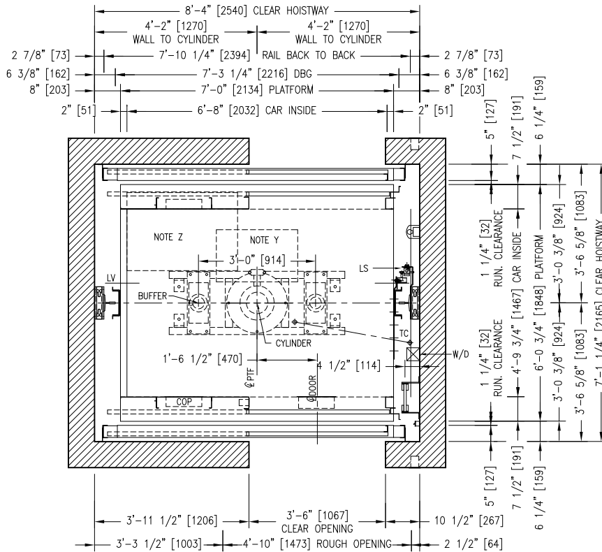
RIGHT HAND
